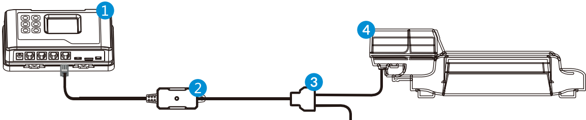
1. Controller 2. Lighting Control Adapter DLI 3. Splitter 4. DLI Ballast
